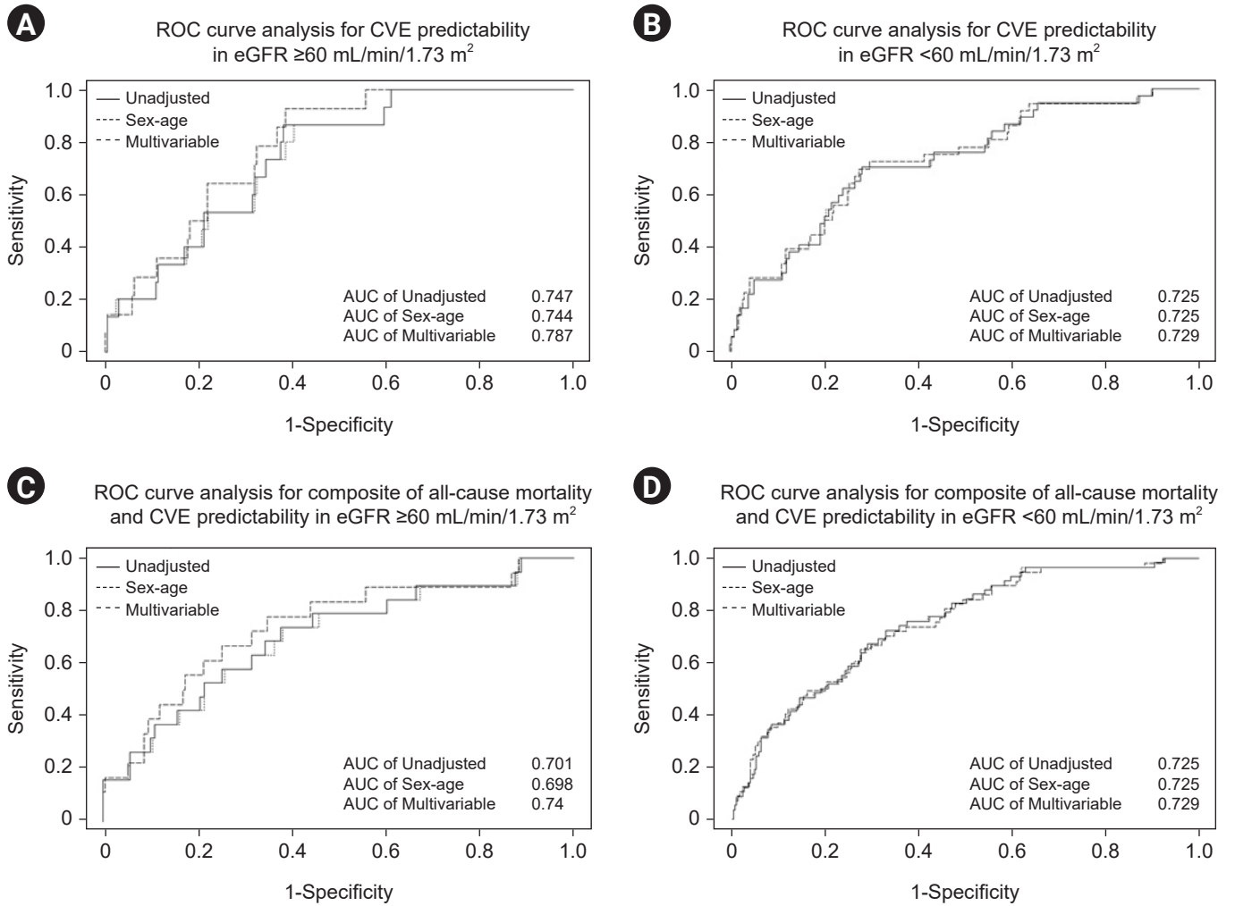
Supplementary Figure 1. Subgroup ROC curve analysis for CVE and composite of all-cause mortality and CVE predictability.
