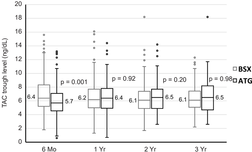
Supplementary Figure 3. Tacrolimus trough levels after kidney transplantation. TAC trough levels were compared from 6 months after kidney transplant and onwards because the KOTRY collected them at discharge during late period of this study. ATG, antithymocyte globulin; BSX, basiliximab; KOTRY, Korean Organ Transplantation Registry; TAC, tacrolimus
